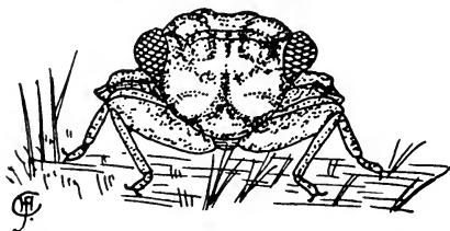
Fig. 360. Cephalic view of a toad bug, Gelastocoris oculatus (Fabr.)
